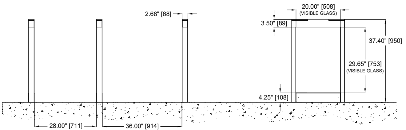
Elevation View
